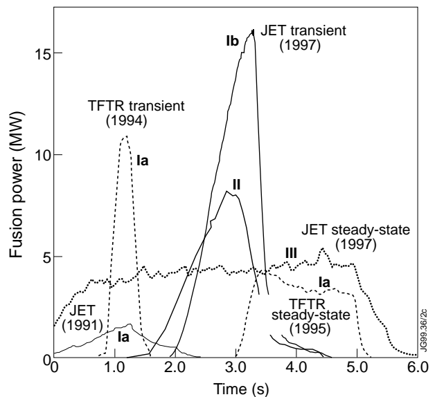
Fig. III Fusion power development in the D-T campaigns of JET (full and dotted lines) and TFTR (dashed lines), in different regimes: (Ia) Hot-Ion Mode in limiter plasma (Ib) Hot-ion H-Mode, (II) Optimized shear and (III) Steady-state ELMY-H Modes [21b].
